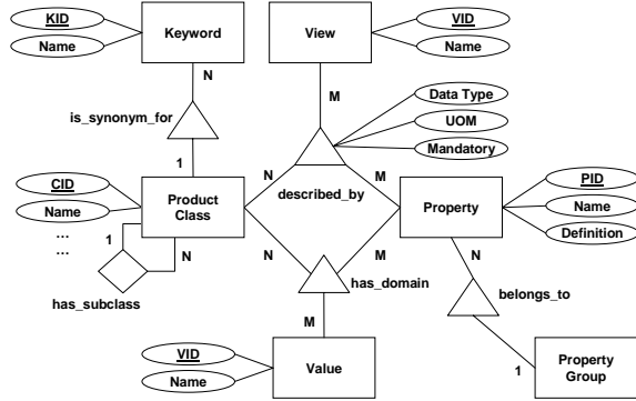
Figure 2: Modified conceptual model.
