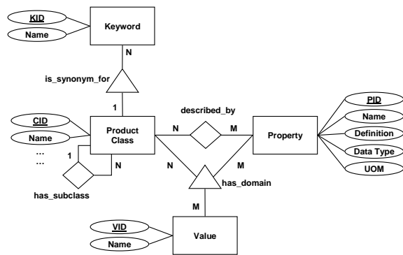
Figure 1: Basic conceptual model.
